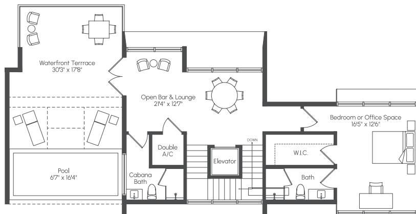
LEVEL 4
